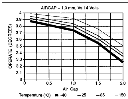
Figure 5-31 Operate Point vs. Air Gap
