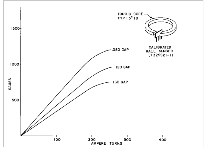
Figure C-32 Effect of gap on typical ferrite toroid core
